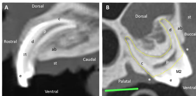
Figure 1. The CT images of a representative incisor and molar. A: Mandibular first incisor (I1), sagittal view showing the uneven distribution of enamel, with most of the enamel on the rostral surface. B: Maxillary second molar (M2), mesial transverse view. Enamel (e) and cementum (c) are bright white. Dentin (d) and alveolar bone (ab) are light grey. Soft tissue (st) and tooth root pulp (p) are darker grey. The green bar is the scale bar (1 cm) for scale calibration. The tooth root area (outlined in yellow) was calculated by tracing the tooth root outline from the buccal to the palatal/lingual cemento-enamel junction (*).
